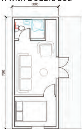
Gelli Pod - floor plan
